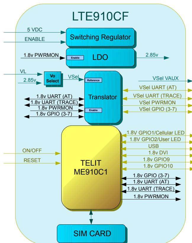
Figure 1 LTE910CF CAT-M1 Block Diagram
