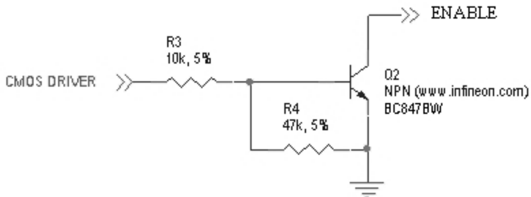
Figure 5 Enable Pin
