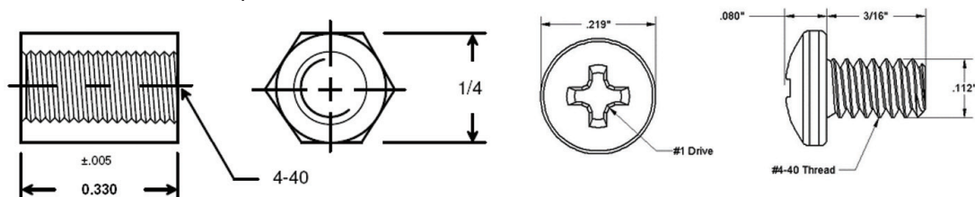
Figure 9 Screw Diagram
